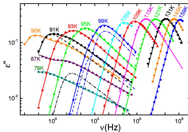
FIG. 1. (Color online) Dielectric loss for the compound Freon112. The lines show the fits using two ( 79 < T < 130 K) or one ( 130 < T < 160 K) CD functions used to fit the spectra in the first temperature range are indicated for 91 and 99 K by the dashed and dot-dashed lines.
