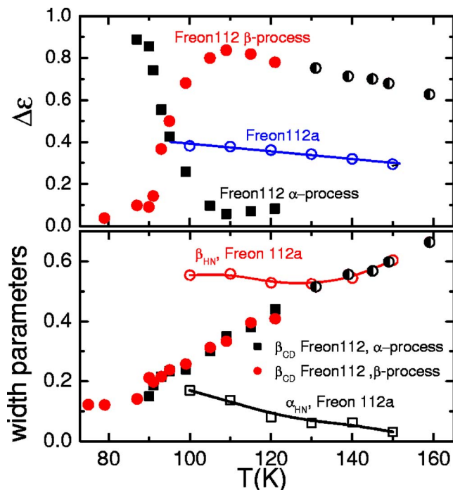
FIG. 3. (Color online) Relaxation strength and width parameters used to fit the Freon112 and Freon112a spectra. The parameters used to fit the single high temperature \alpha\beta relaxation peak for Freon112 are shown as half-filled circles. The lines are drawn to guide the eyes.
