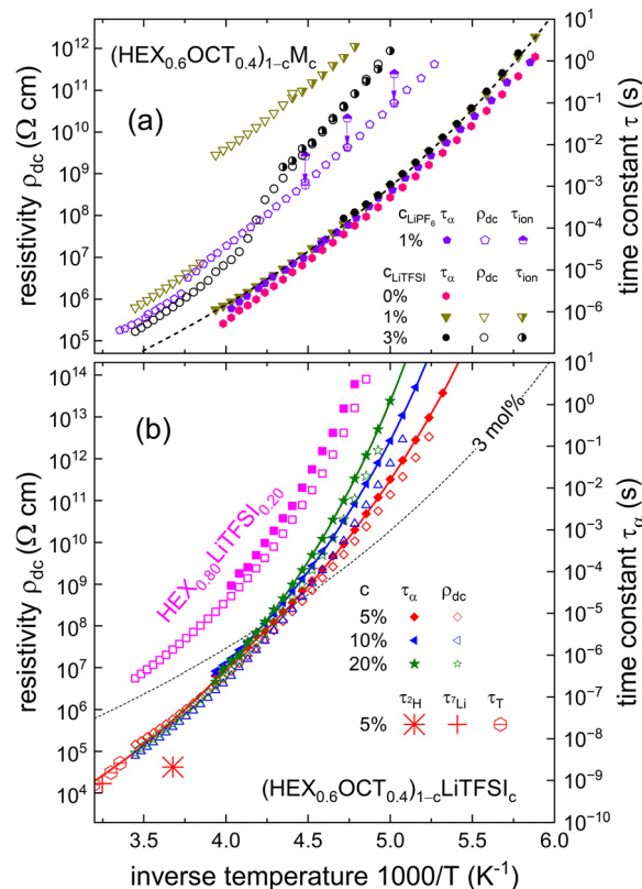
Fig. 6 Arrhenius plot of resistivity \rho_{dc} (open symbols) and relaxation times ( \tau_\alpha as filled symbols and \tau_{ion} as half-filled symbols, both derived from inverse circular peak frequencies) for \text{HEX}_{0.6}\text{OCT}_{0.4} doped (a) at mole fractions (a) of c < 5 mol% and (b) at larger levels. Frame (a) features data relating to LiTFSI doping as well as results of a sample devoid of added salt. The purple pentagons represent data (based on ref. 25) for a crystal doped with 1 mol% of \text{LiPF}_6 . In frame (a), the ordinate axes are shifted so that for (\text{HEX}_{0.6}\text{OCT}_{0.4})_{0.97}(\text{LiTFSI})_{0.03} the \tau_{ion} and the \rho_{dc} data overlap. Frame (b) shows \rho_{dc} and \tau_\alpha for (\text{HEX}_{0.6}\text{OCT}_{0.4})_{1-c}(\text{LiTFSI})_c with c = 5, 10 , and 20 mol% as well as for \text{HEX}_{0.80}\text{LiTFSI}_{0.20} . For visual clarity, the latter data are shifted upward by 2 decades. Also included are NMR-based motional times inferred from the ^2\text{H} (asterisk) and ^7\text{Li} (plus sign) T_1 minima reported in Fig. 4, as well as the diffusion-based translational times \tau_T (hexagons with horizontal bars). All lines in the present figure are guides to the eye. In both frames, the y-axes are adjusted so that all decade ticks are spaced equally. Thus, by construction, the relative shift of the \rho_{dc} and the \tau axes in frame (a) differs from that chosen for frame (b).
