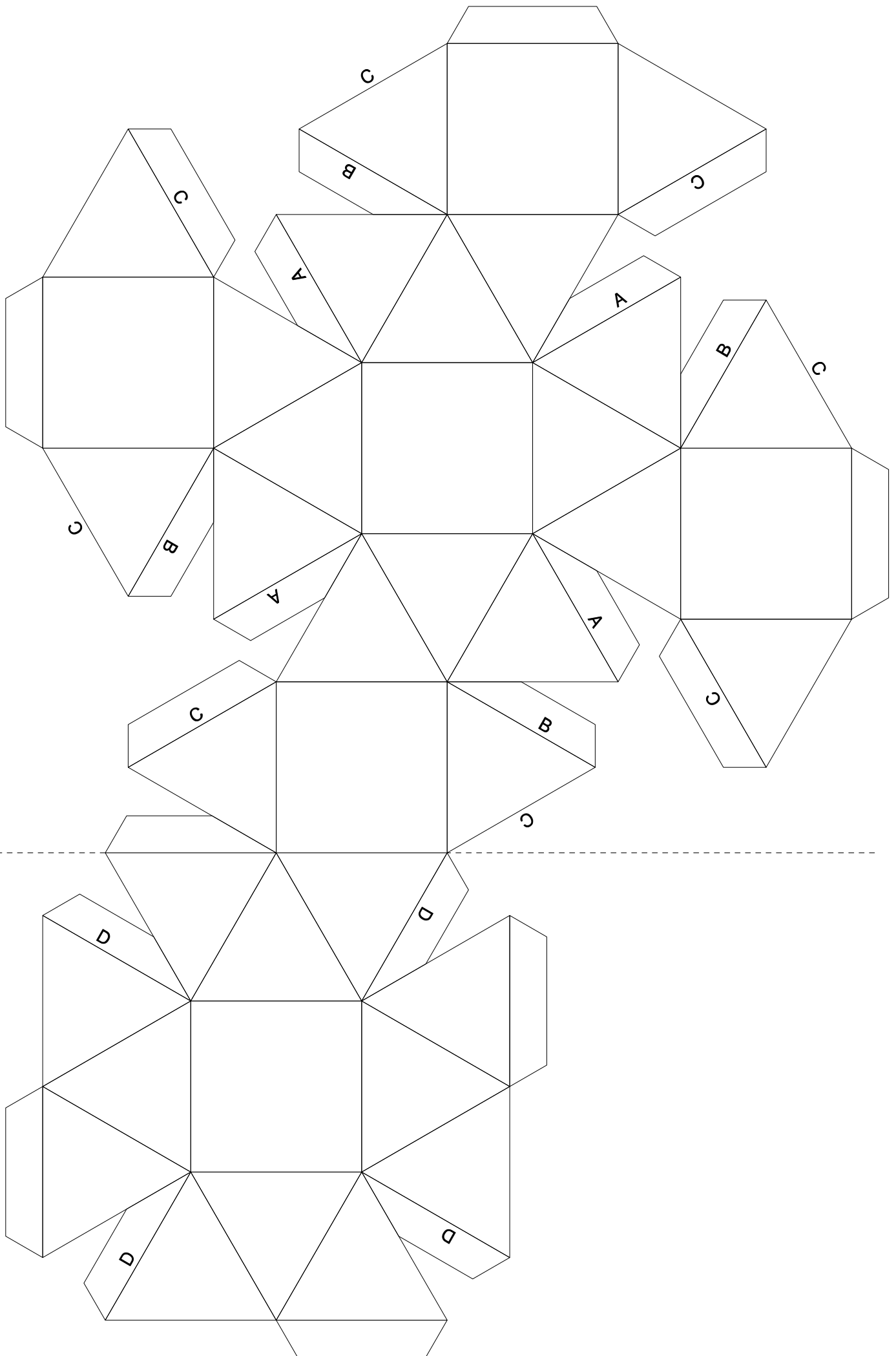
Stumpf-Hexaeder (R) (3,3,3,3,4) ( max. Kante = 3.5 cm )
