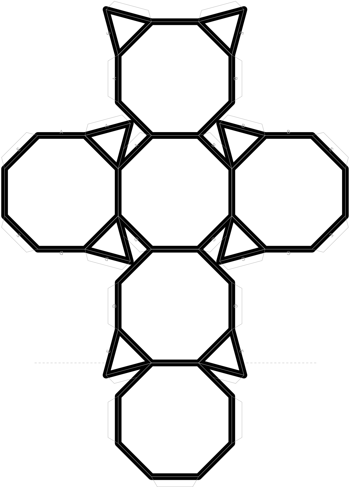
Stutz-Hexaeder (3,8,8) ( max. Kante = 2.5 cm )
