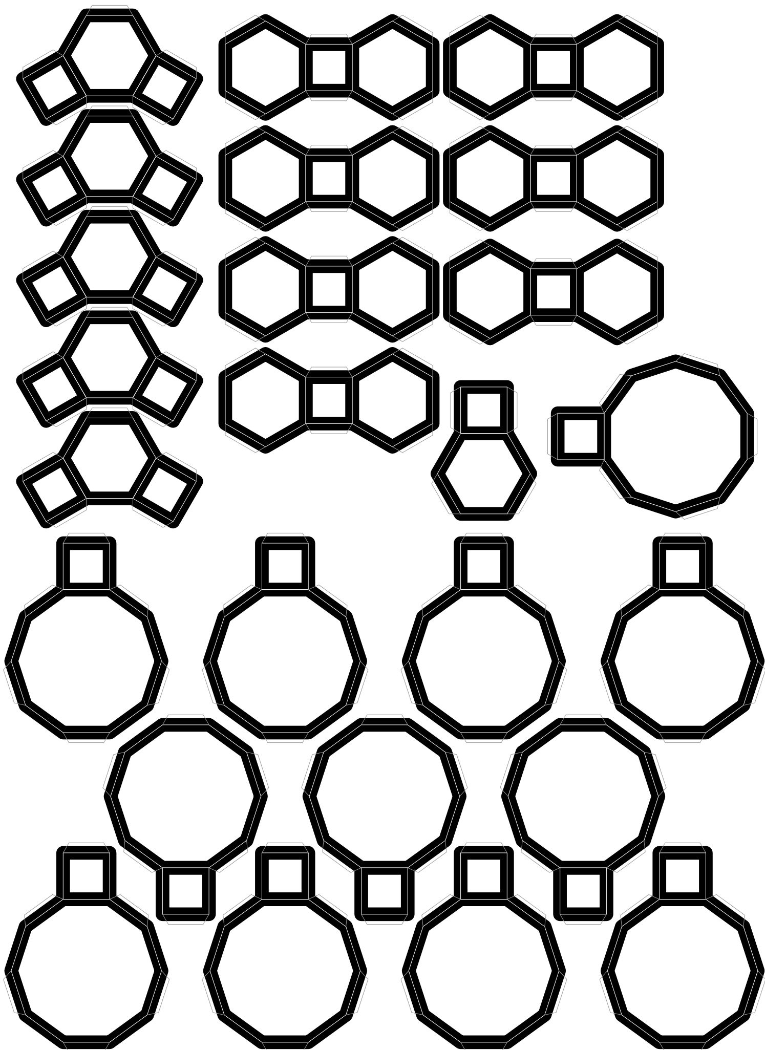
Gross-Rhombikositodekaeder (4,6,10) ( max. Kante = 1.2 cm )
